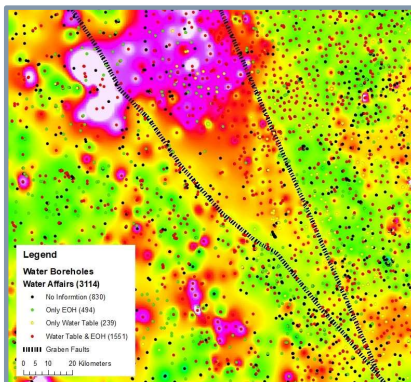
Ground Water Levels
